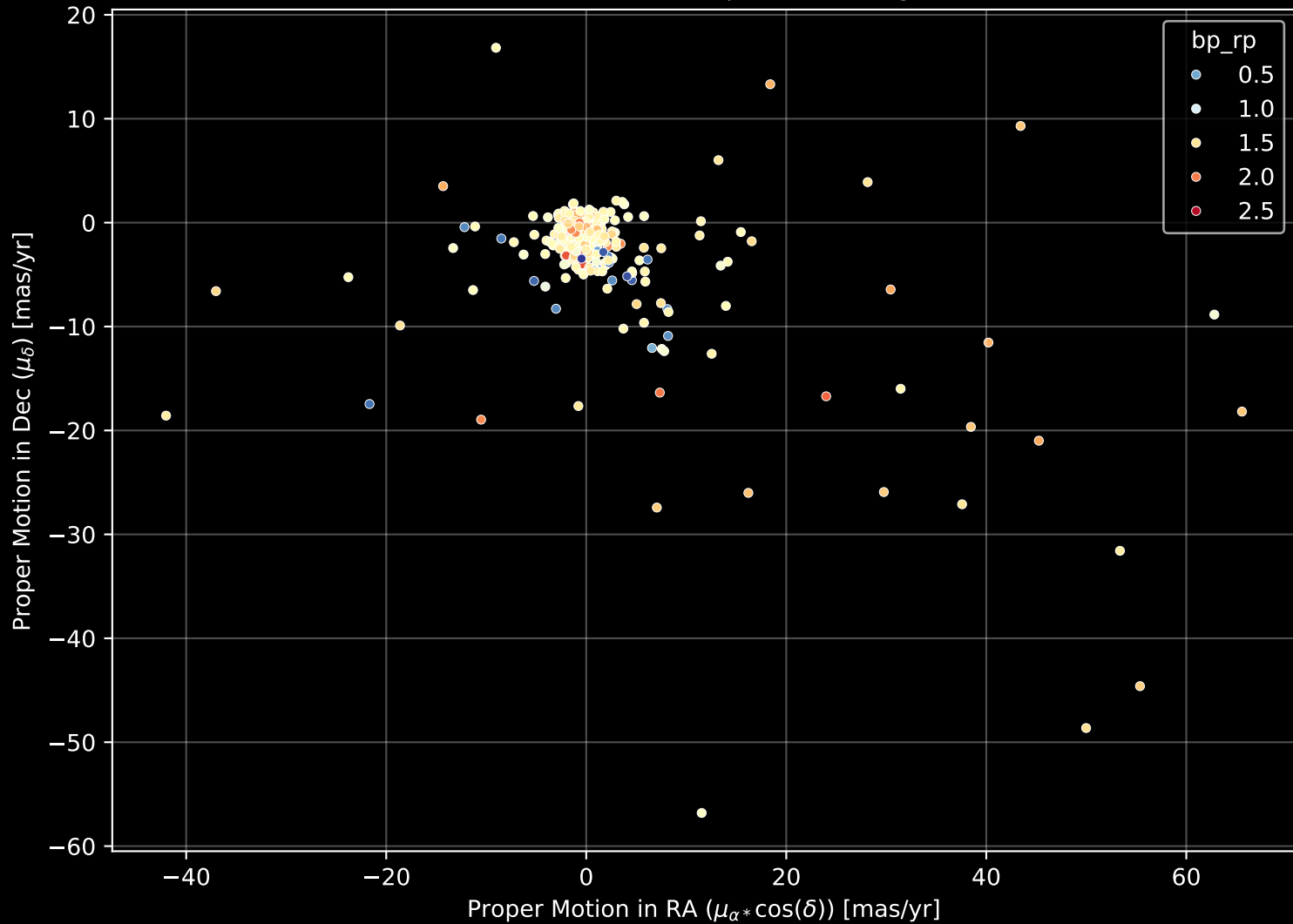
APOGEE DR17 Field: [140-12] Proper Motion Diagram (n= 305)
