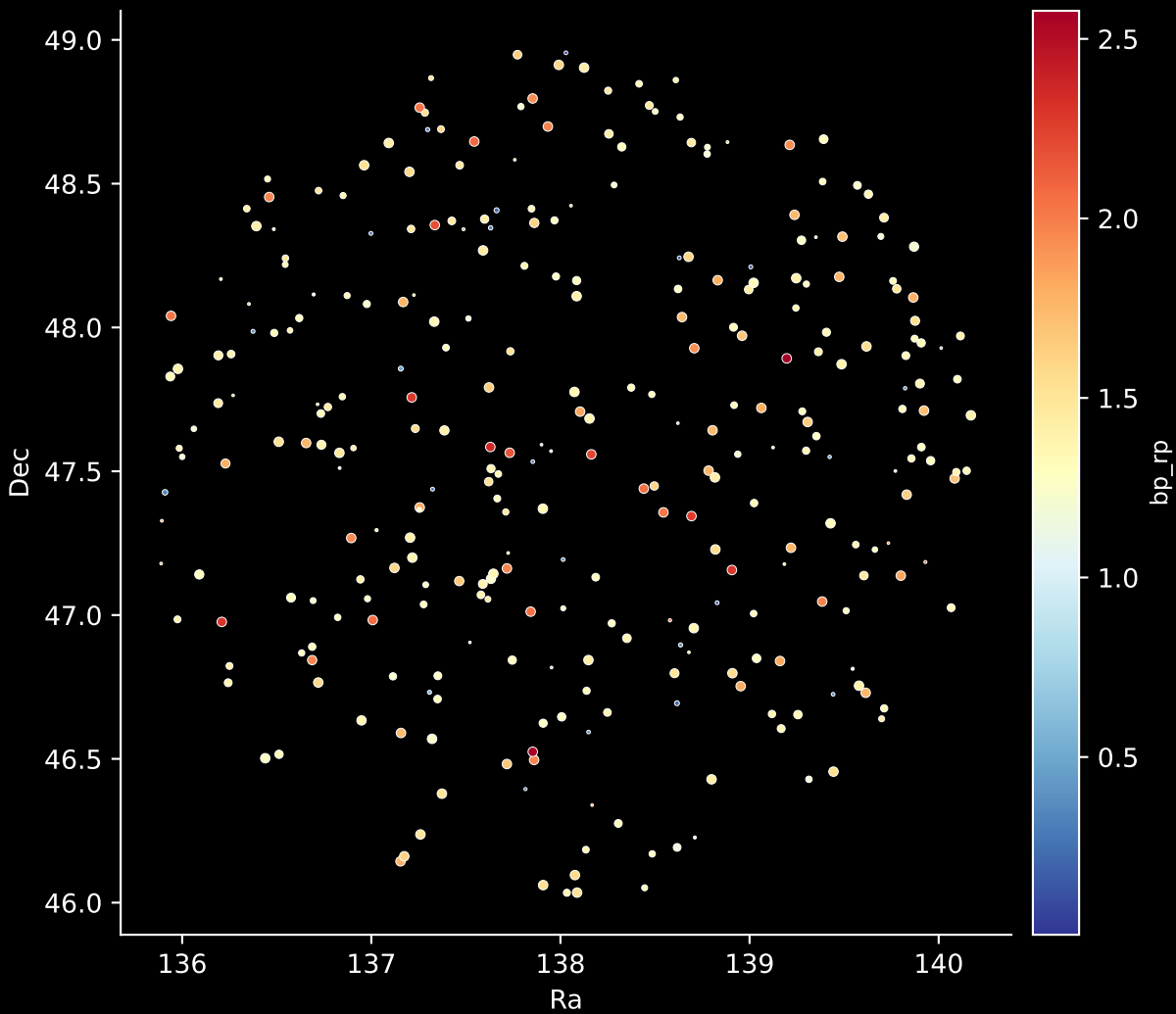
APOGEE DR17 Field: [140-12] Stars: 305
