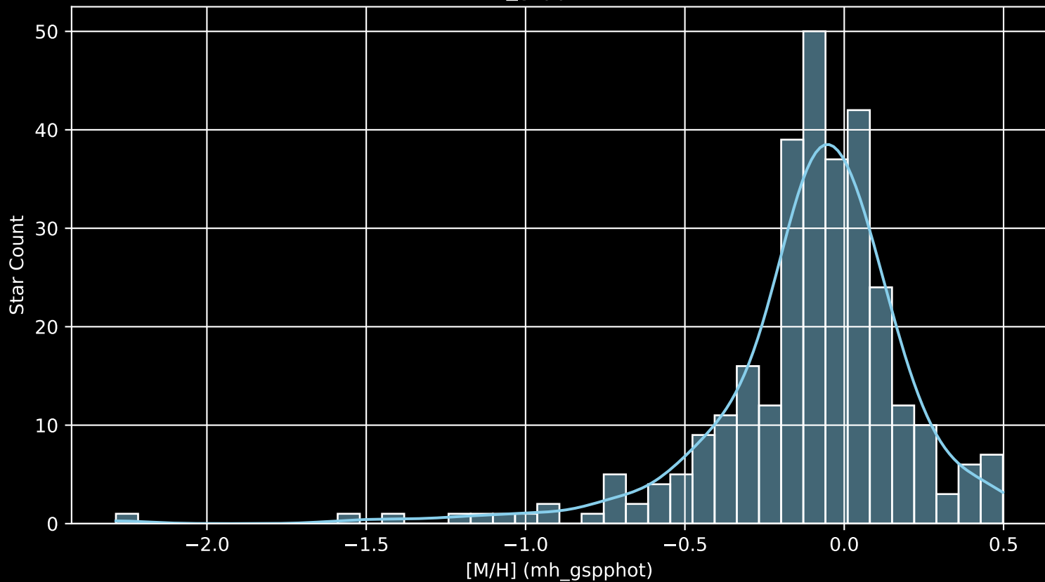
APOGEE DR17 Field: [140-12 [M/H] (mh_gspphot) (n= 304)
