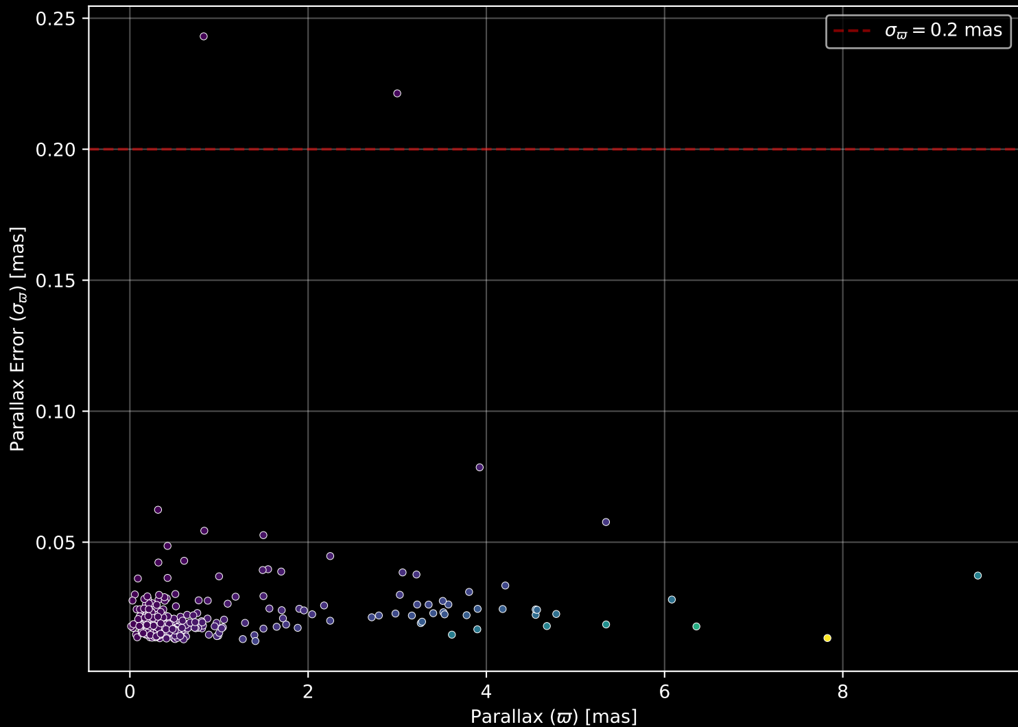
APOGEE DR17 Field: [140-12] Parallax Quality (n= 305)
