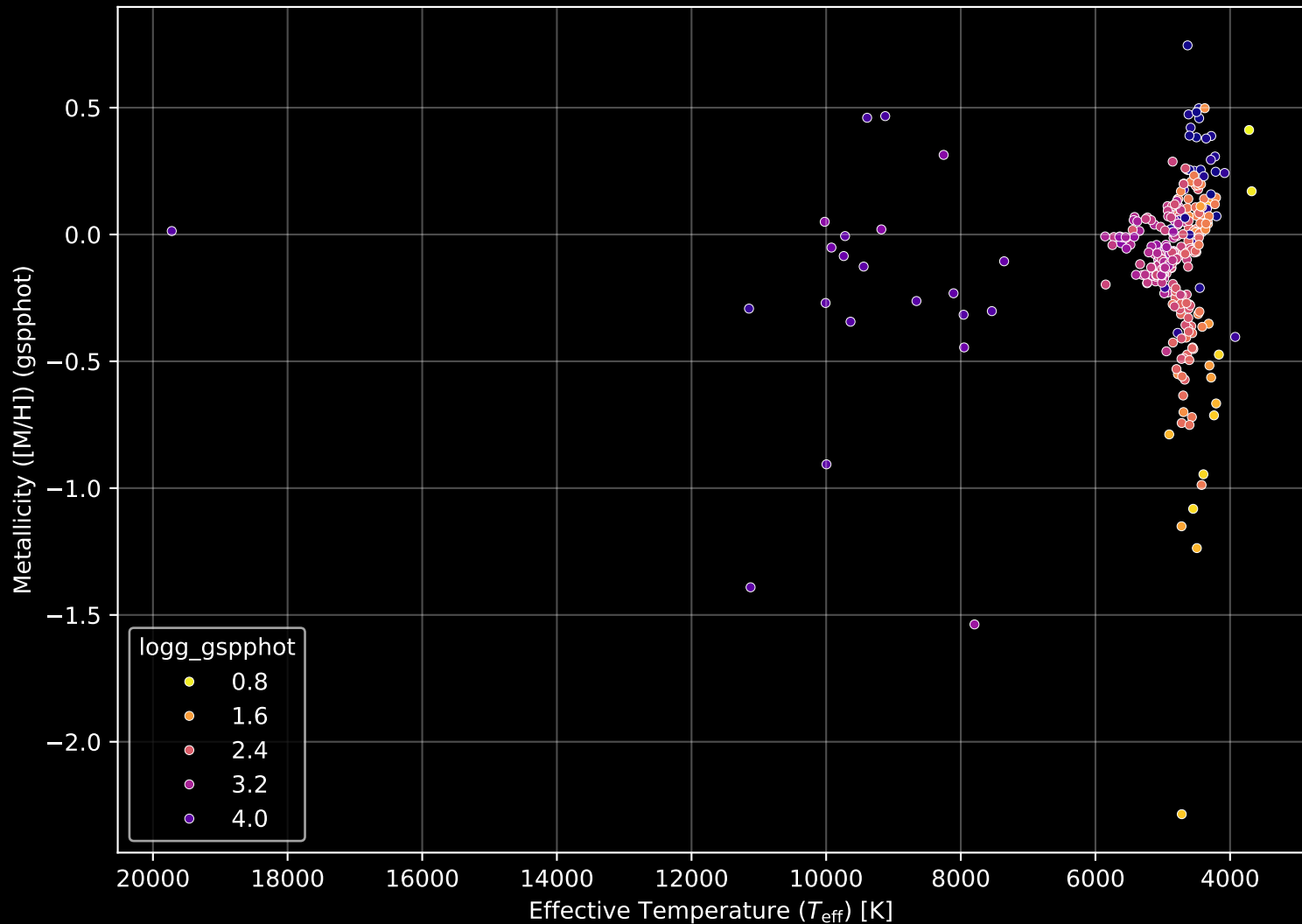
APOGEE DR17 Field: [140-12] Stellar Population Parameters (n= 305)
