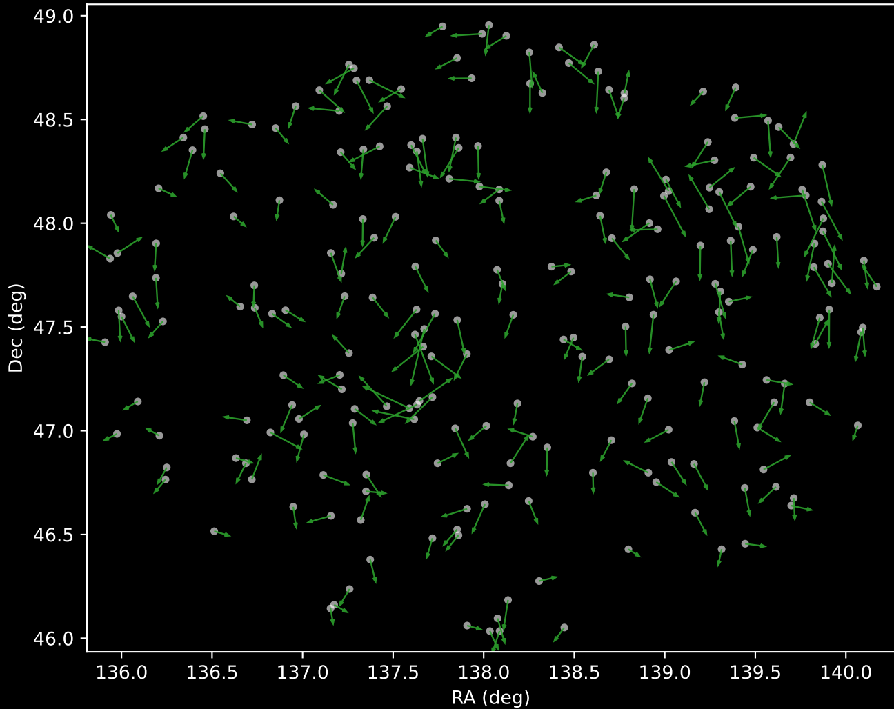
APOGEE DR17 Cluster 4 Proper Motion Vectors (n=231)
