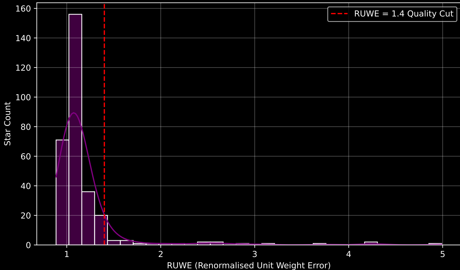
GAPOGEE DR17 Field [140-12] RUWE Distribution (n= 303)
